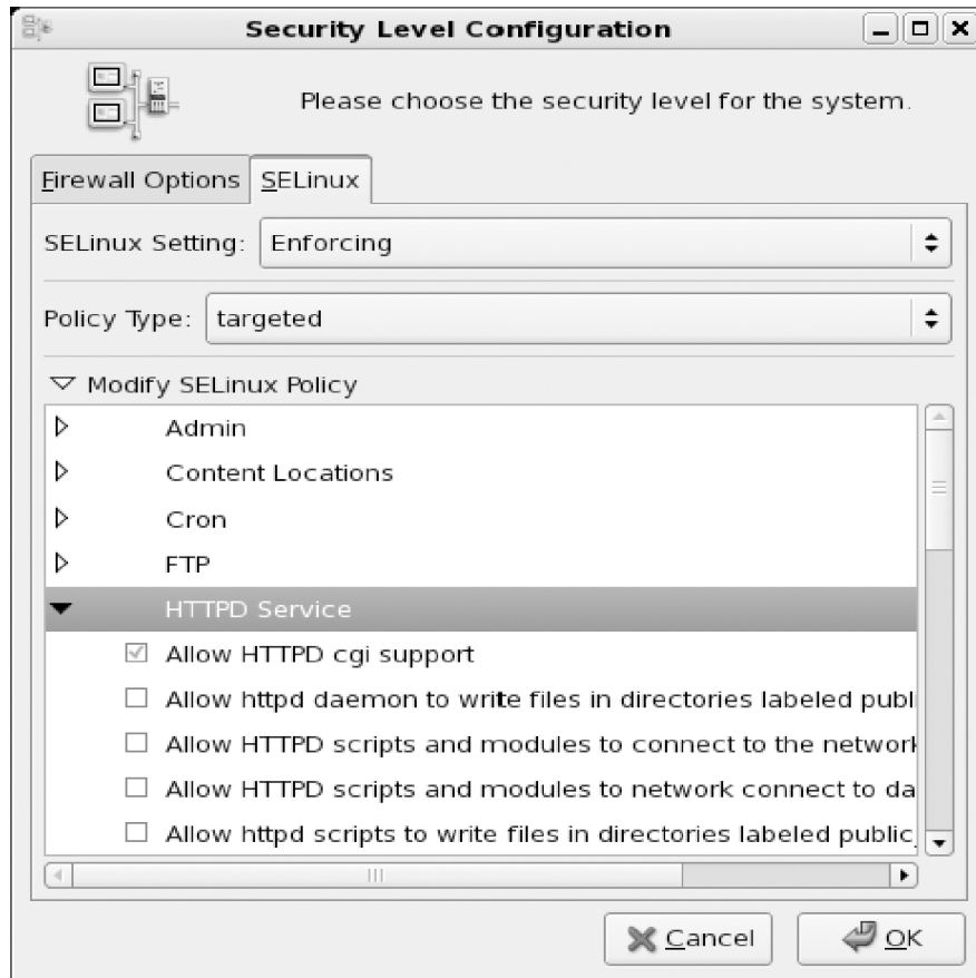
Figure 1. Interface in Fedora for configuring SELinux
